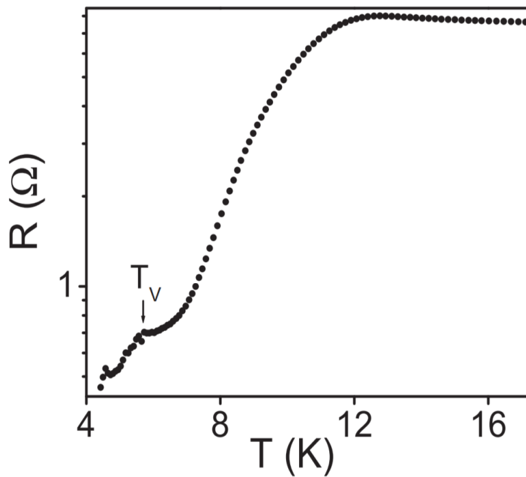
Figure 5.17 Resistance vs Temperature at low (~50 \mu A) current
