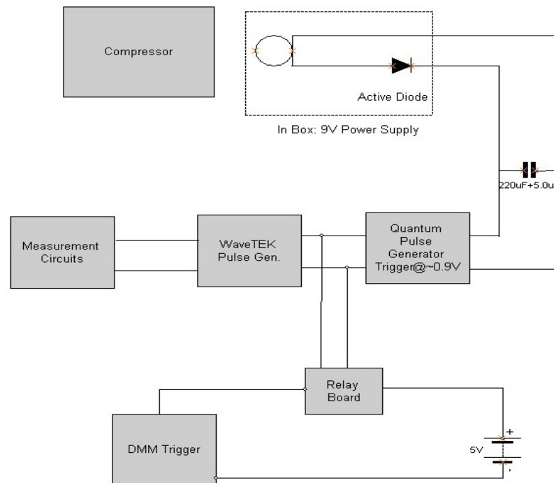
Figure 4.10: Trigger by Sound diagram
