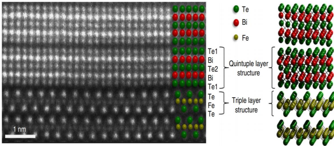
Figure 3.2 HADDF image showing the sharpness of the gap between the two layers
