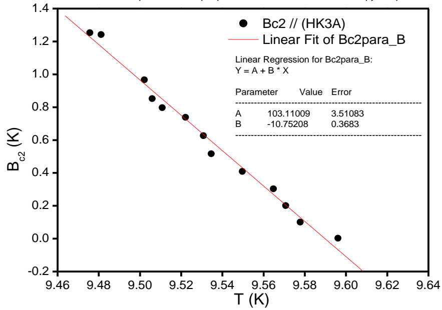
Figure 5.4 Parallel Bc2 vs Temperature, Bc2(0) found to be ~70T
